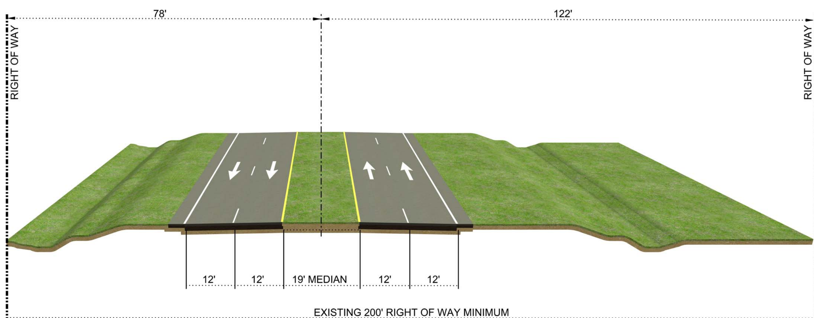
SR 50 (Colonial Dr) Existing Typical Section (4-Lane) From Avalon Park Blvd to SR 520
