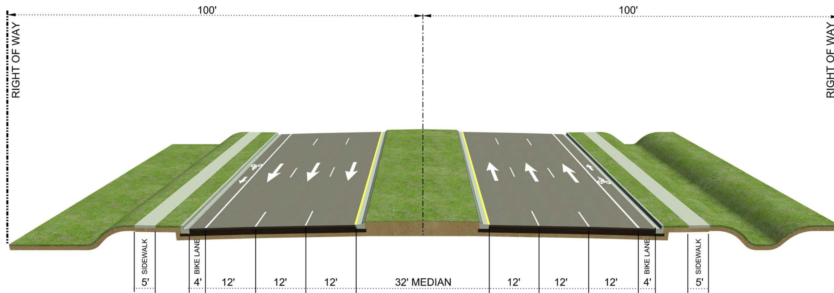
SR 50 (Colonial Dr) Existing Typical Section (6-Lane) From Woodbury Rd to Avalon Park Blvd
